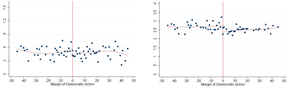
a. Rd Graph - CO (left) and NO2 (right)
