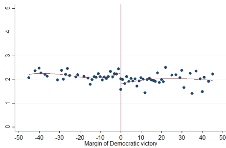
c. Rd Graph - SO2
